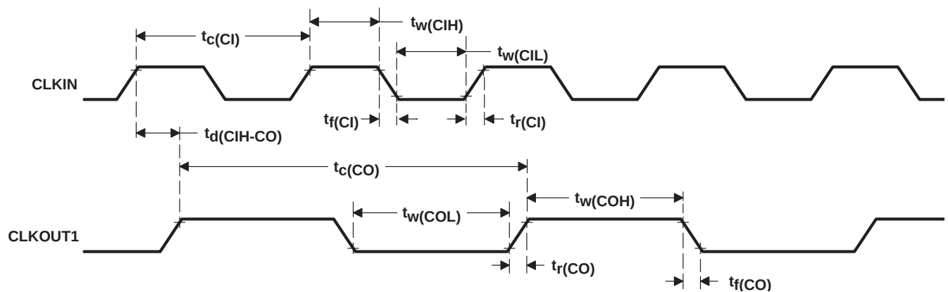
Figure 10. CLKIN-to-CLKOUT1 Timing Without PLL (using \div 2 clock option)
